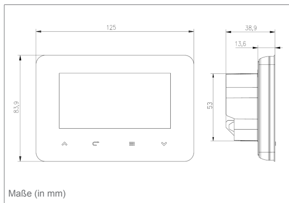
Raumthermostat RT 05 D-230 / RT 05 D-BAT
